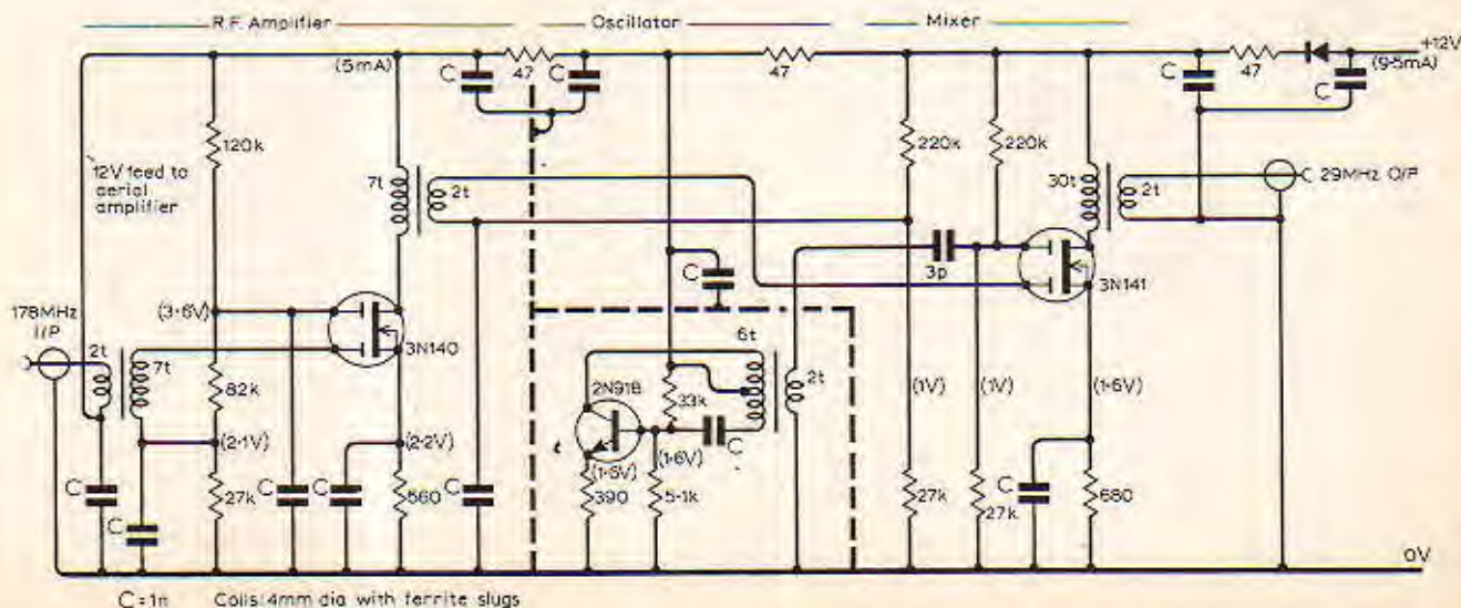
C=1n Coils: 4mm dia with ferrite slugs
