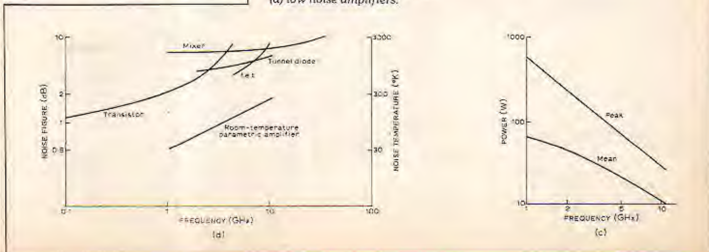
Fig. 5. Typical performance graphs for semiconductor devices now used in m.i.c. technology; (a) microwave power transistor, (b) impatt oscillator, (c) trapatt oscillator, (d) low noise amplifiers.
